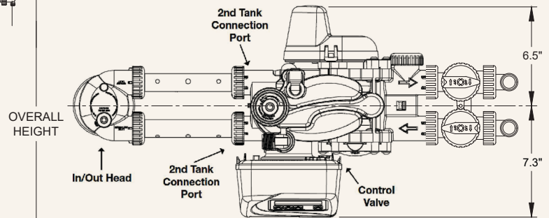
ENLARGED TOP VIEW SHOWN WITH BYPASS AND 1.0 MNPT ELBOWS
