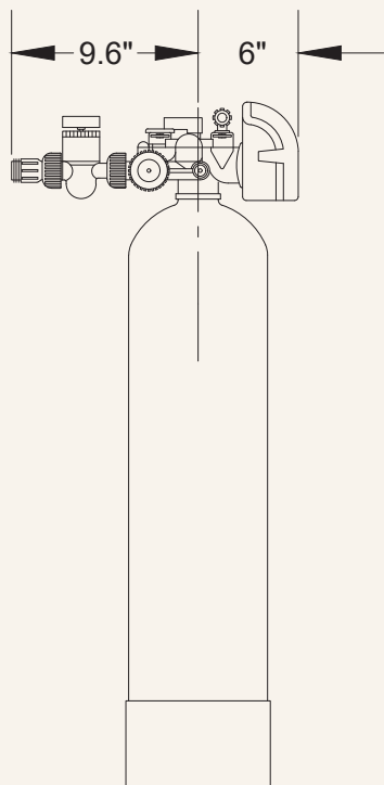
OUTLET SIDE VIEW SHOWN WITH BYPASS AND 1.25 MNPT ASSEMBLY
