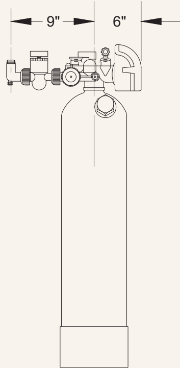
OUTLET SIDE VIEW SHOWN WITH BYPASS, 1.0 MNPT ELBOW ASSEMBLY AND TANK DOME PLUG
